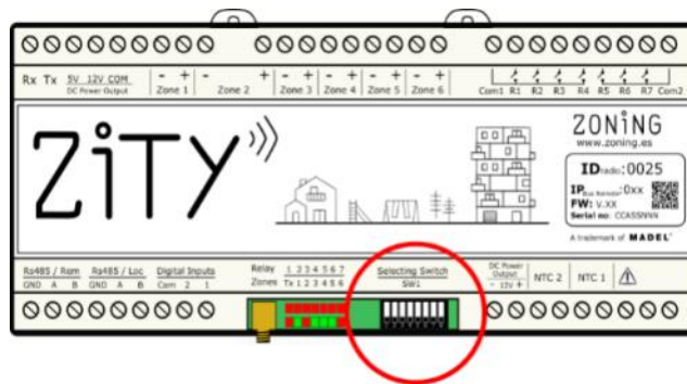
Selecting Switch SW1
